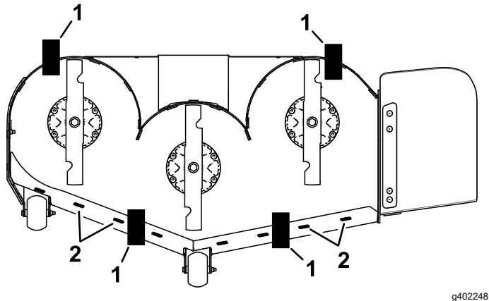
Figure 92 Bottom view
